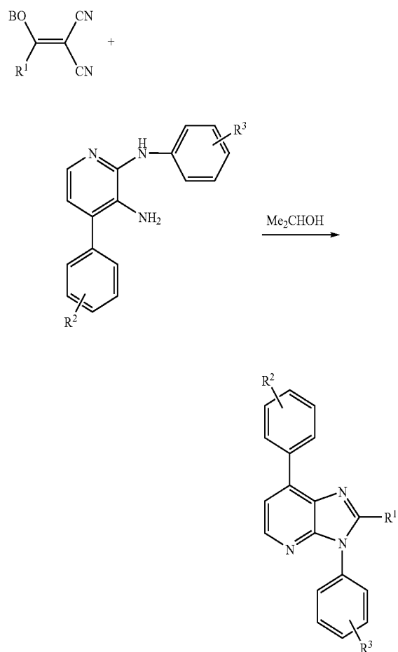
[Reaction Scheme 1]
